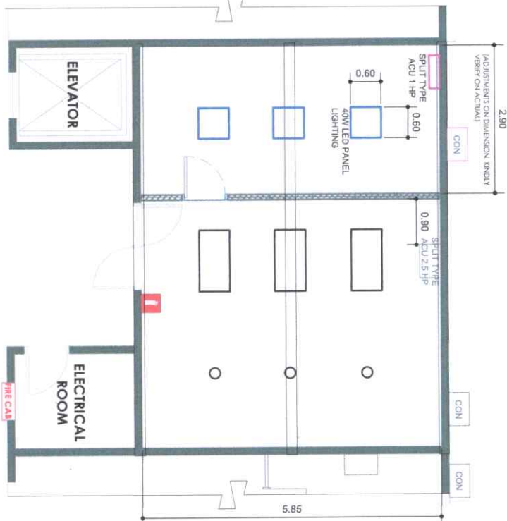
PROPOSED LIGHTING LAY-OUT SCALE 1:100M
